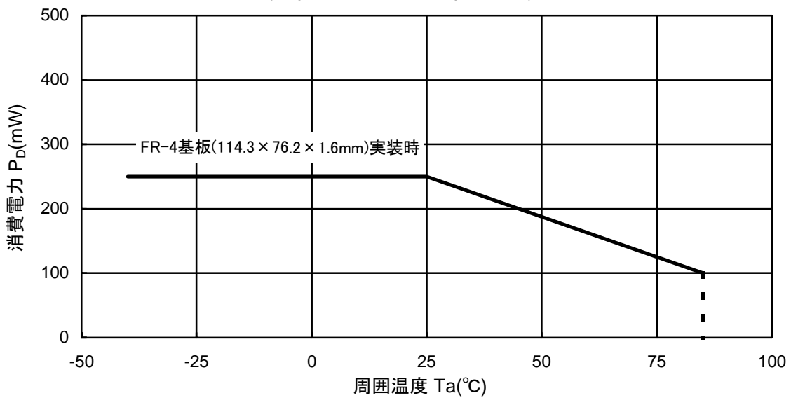
NJM2865F3 消費電力特性例 ( T_{opr}=-40\sim+85^{\circ}\text{C} , T_j=125^{\circ}\text{C} )
