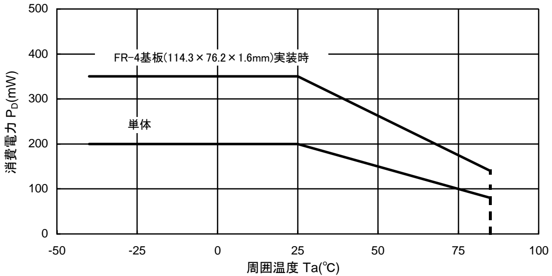
NJM2865/66F 消費電力特性例 ( T_{opr}=-40\sim+85^{\circ}\text{C} , T_j=125^{\circ}\text{C} )
